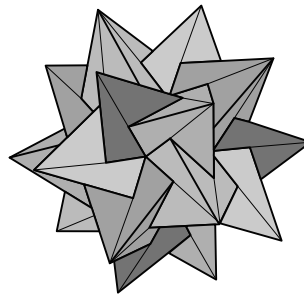
Compound of 5 Tetrahedra Page 63 4" squares of printer paper, 60 sheets. Finished height ~6.5" (A)
